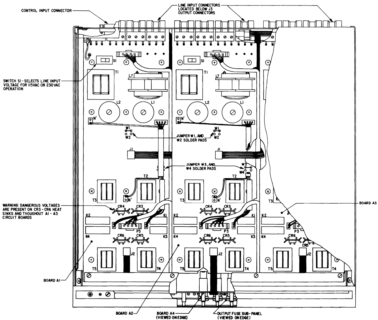
Figure 7-2A. Assembly Locations.
